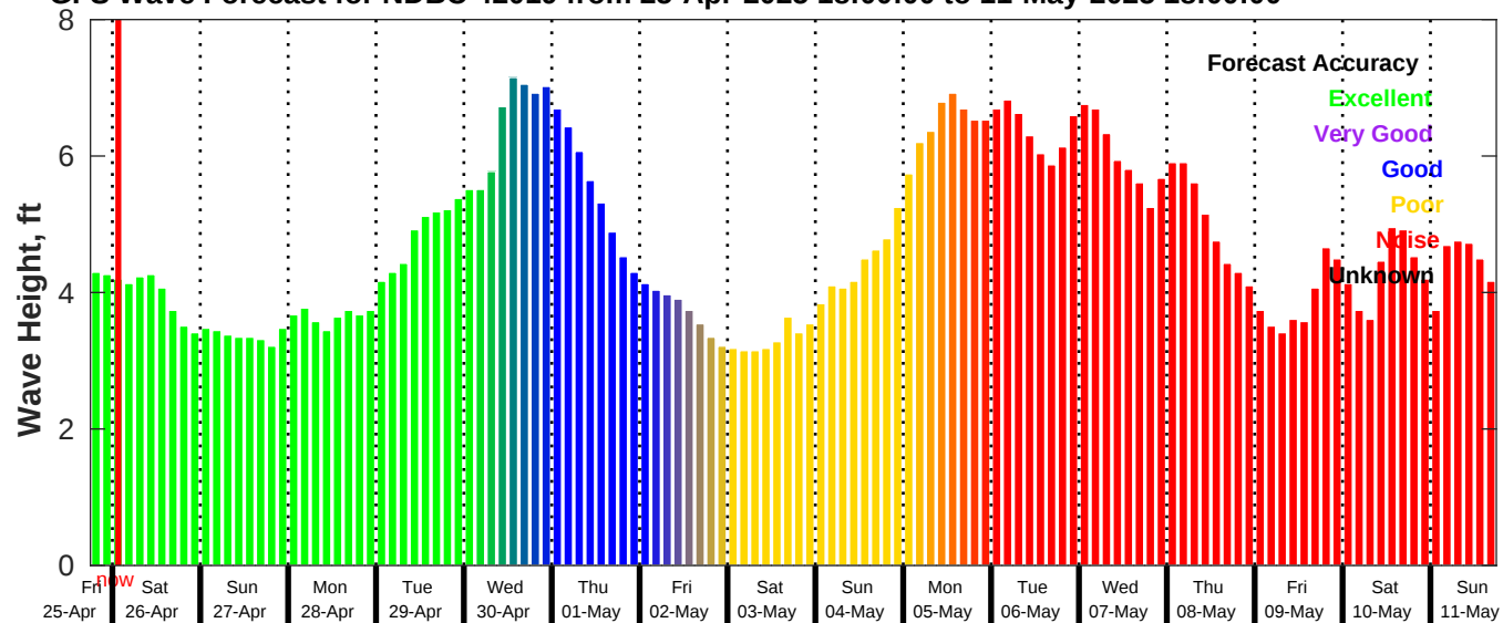
GFS Wave Forecast for NDBC 42019 from 25-Apr-2025 18:00:00 to 11-May-2025 18:00:00
