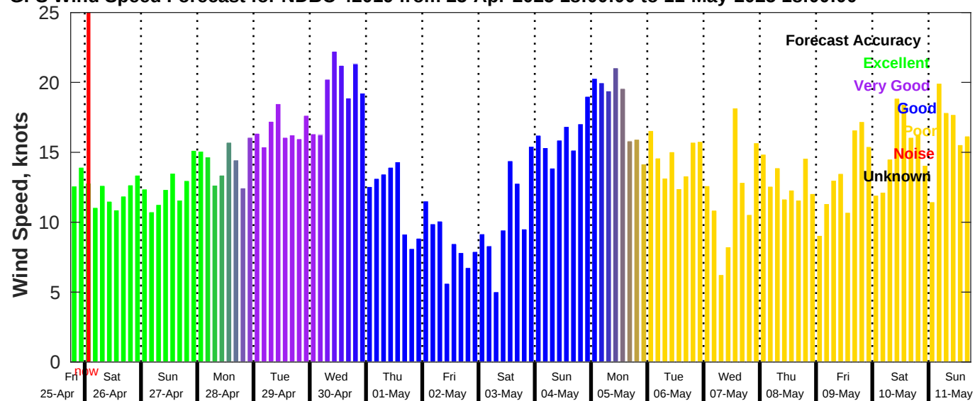
GFS Wind Speed Forecast for NDBC 42019 from 25-Apr-2025 18:00:00 to 11-May-2025 18:00:00
