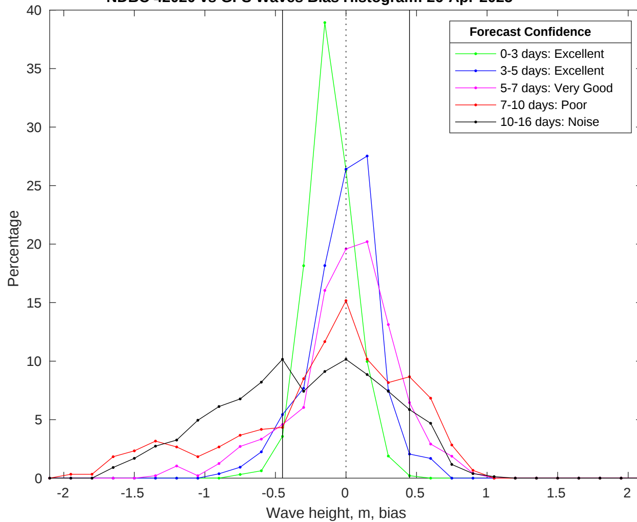
NDBC 42020 vs GFS Waves Bias Histogram: 26-Apr-2025
