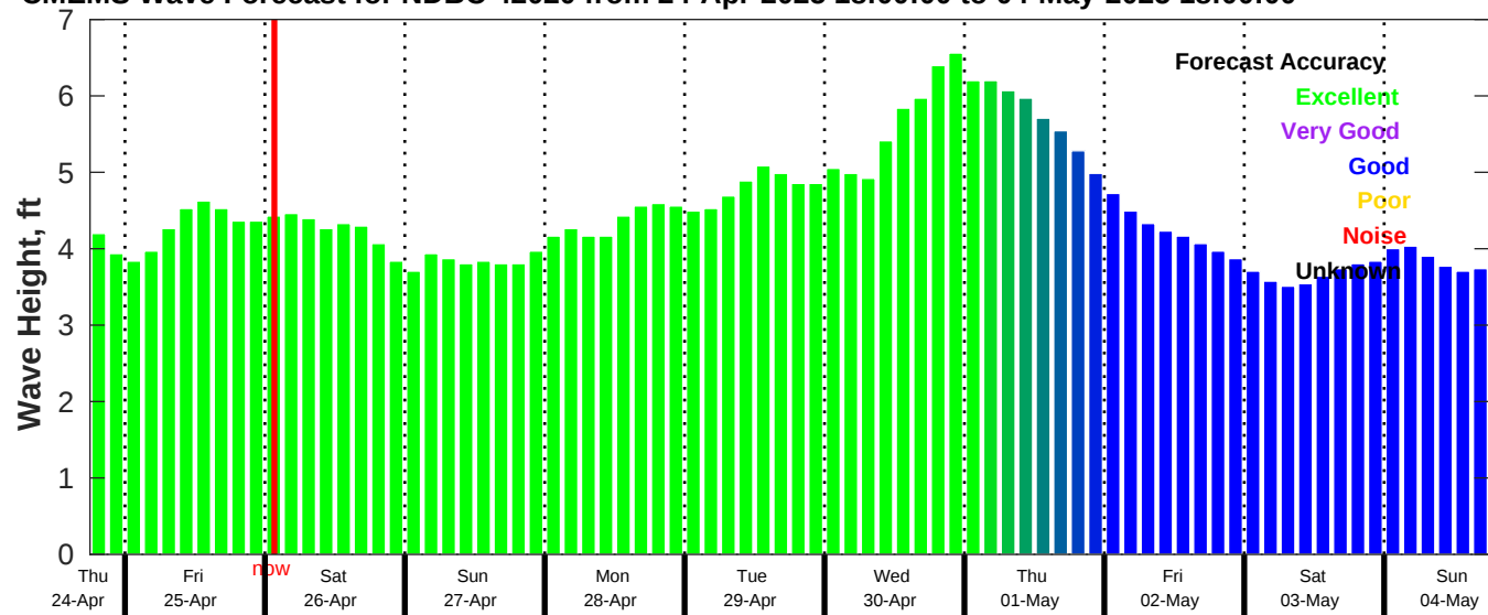
CMEMS Wave Forecast for NDBC 42020 from 24-Apr-2025 18:00:00 to 04-May-2025 18:00:00
