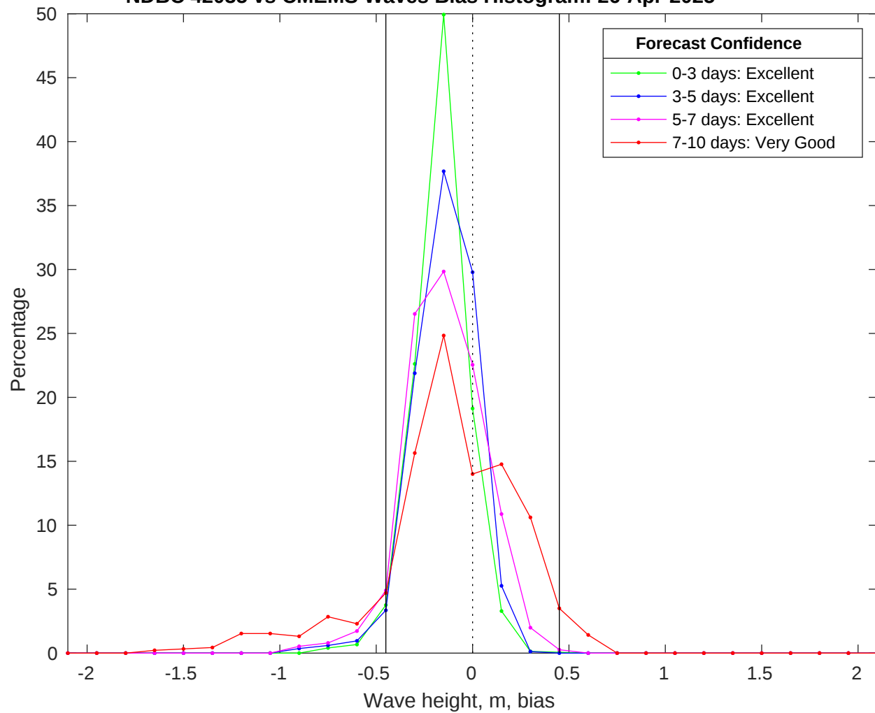
NDBC 42035 vs CMEMS Waves Bias Histogram: 26-Apr-2025
