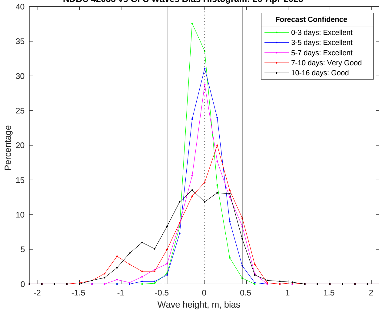
NDBC 42035 vs GFS Waves Bias Histogram: 26-Apr-2025
