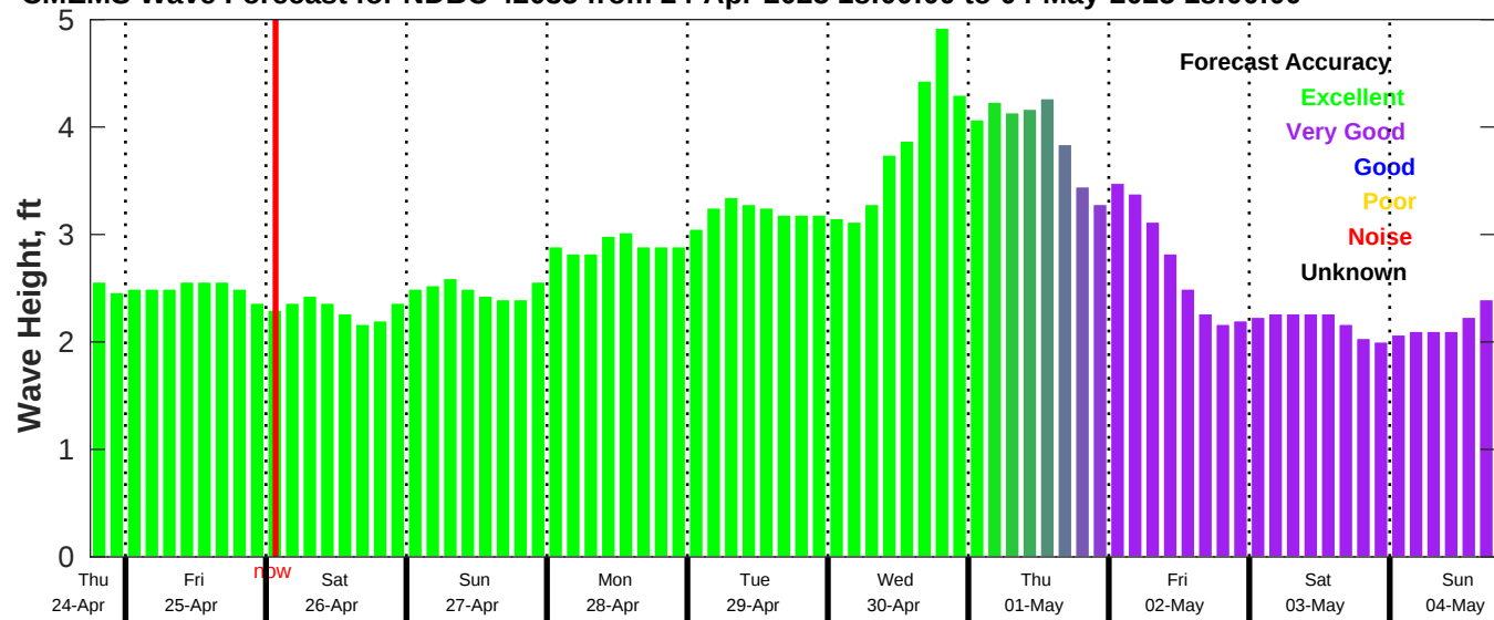
CMEMS Wave Forecast for NDBC 42035 from 24-Apr-2025 18:00:00 to 04-May-2025 18:00:00
