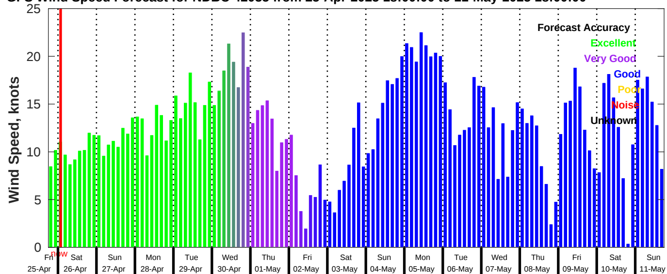
GFS Wind Speed Forecast for NDBC 42035 from 25-Apr-2025 18:00:00 to 11-May-2025 18:00:00
