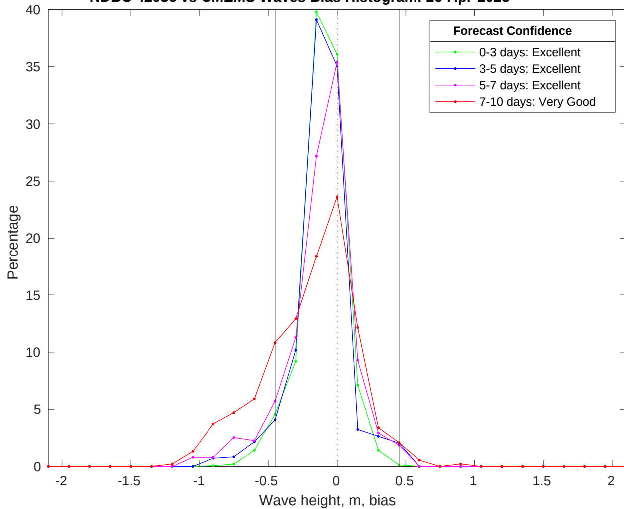
NDBC 42036 vs CMEMS Waves Bias Histogram: 26-Apr-2025
