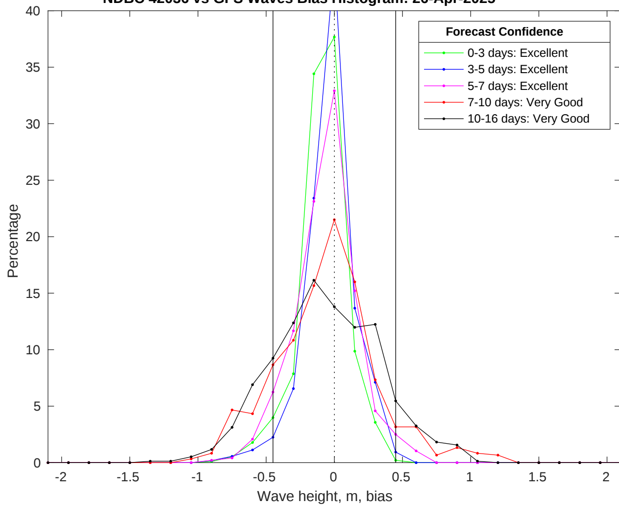
NDBC 42036 vs GFS Waves Bias Histogram: 26-Apr-2025
