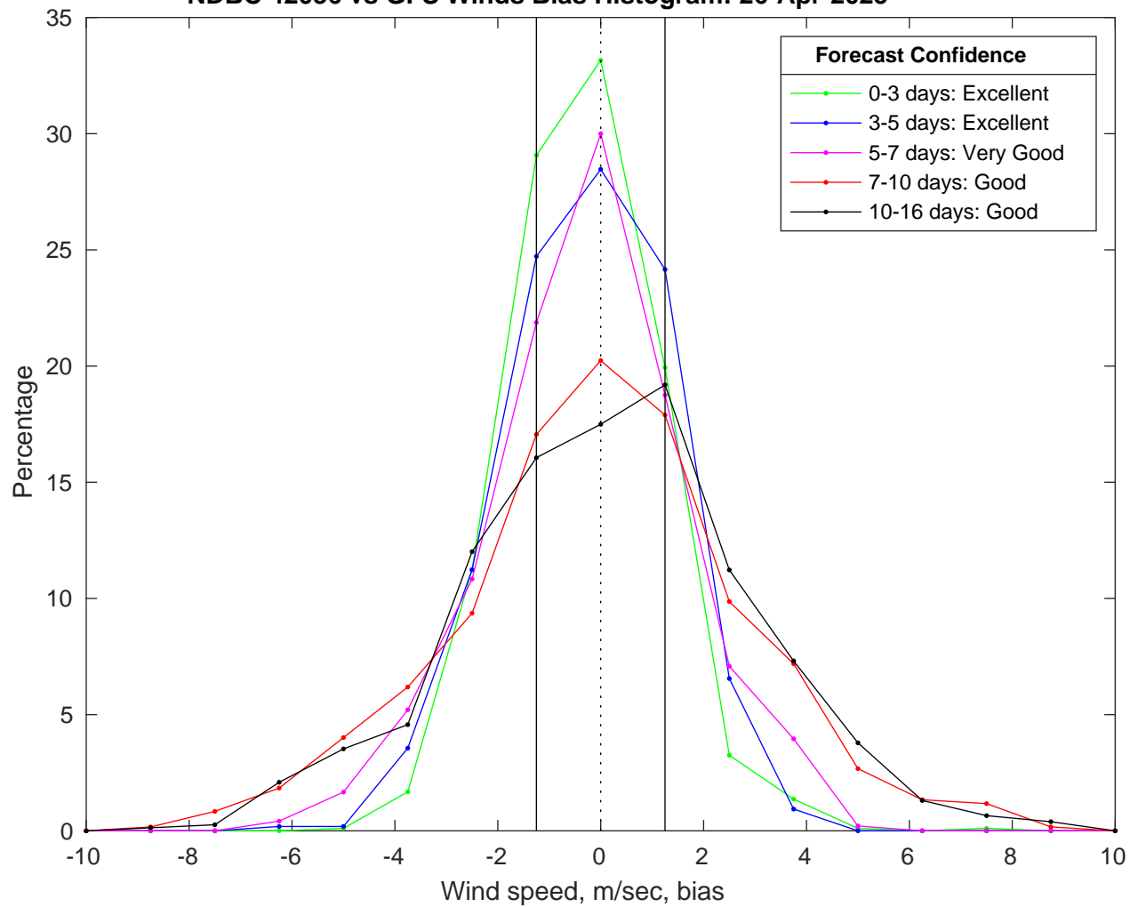
NDBC 42036 vs GFS Winds Bias Histogram: 26-Apr-2025
