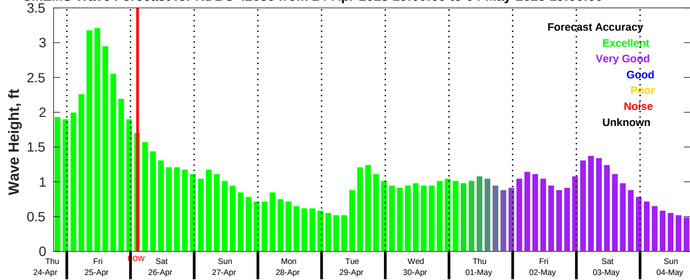
CMEMS Wave Forecast for NDBC 42036 from 24-Apr-2025 19:00:00 to 04-May-2025 19:00:00
