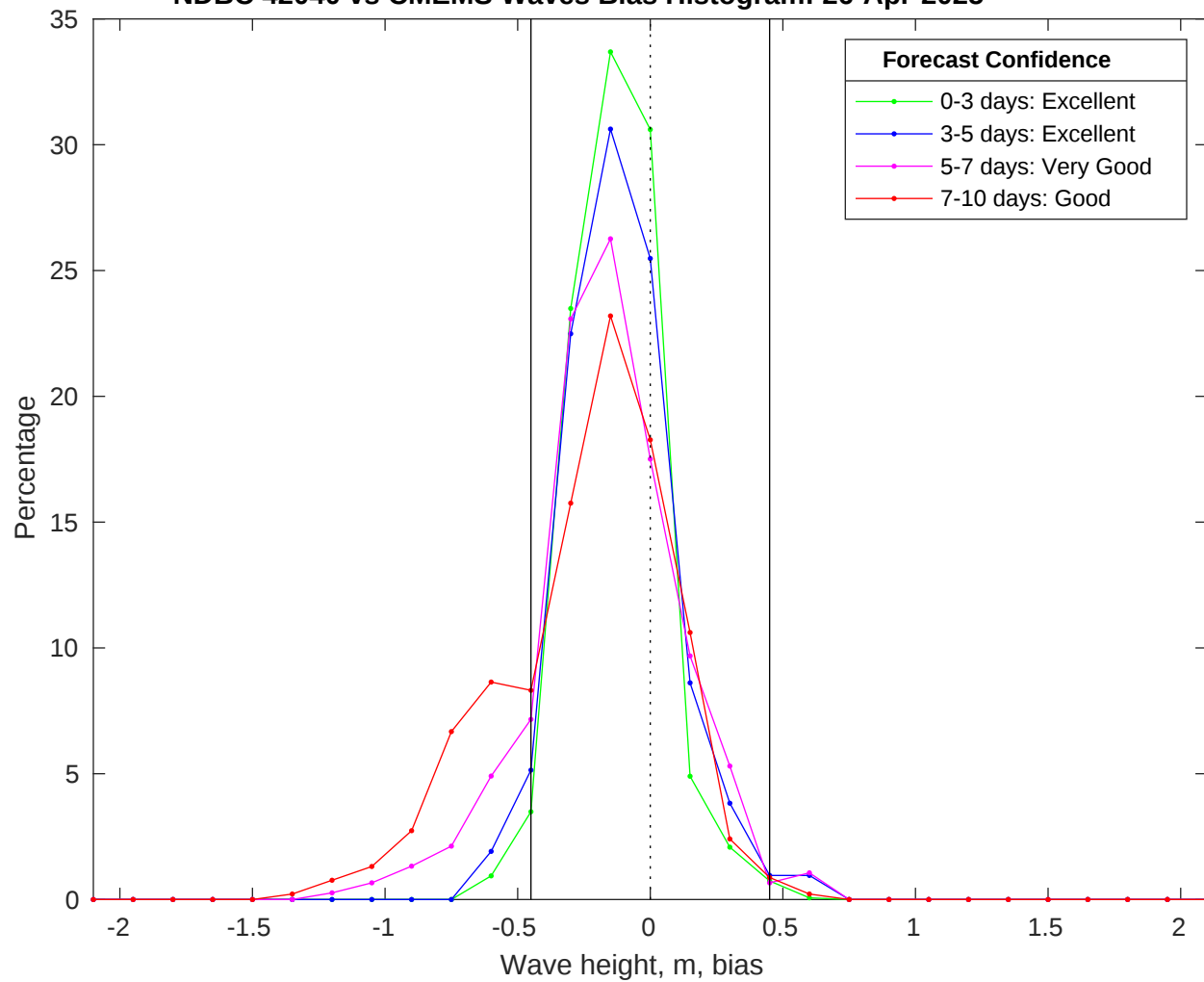
NDBC 42040 vs CMEMS Waves Bias Histogram: 26-Apr-2025
