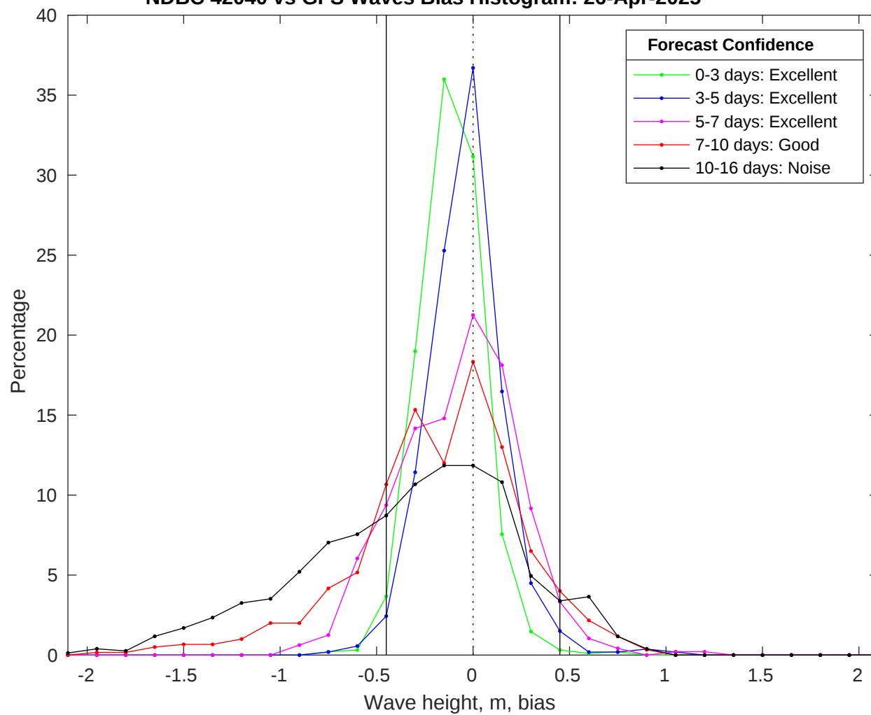
NDBC 42040 vs GFS Waves Bias Histogram: 26-Apr-2025
