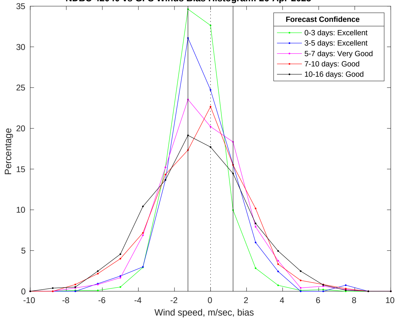
NDBC 42040 vs GFS Winds Bias Histogram: 26-Apr-2025
