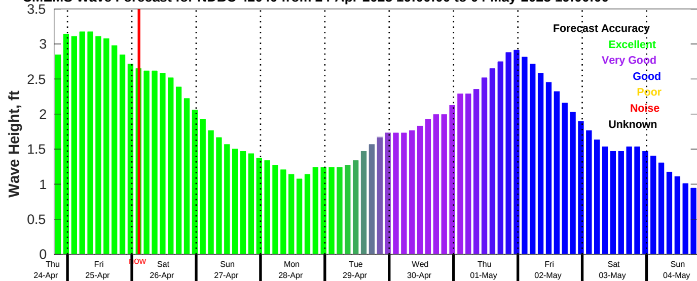
CMEMS Wave Forecast for NDBC 42040 from 24-Apr-2025 19:00:00 to 04-May-2025 19:00:00
