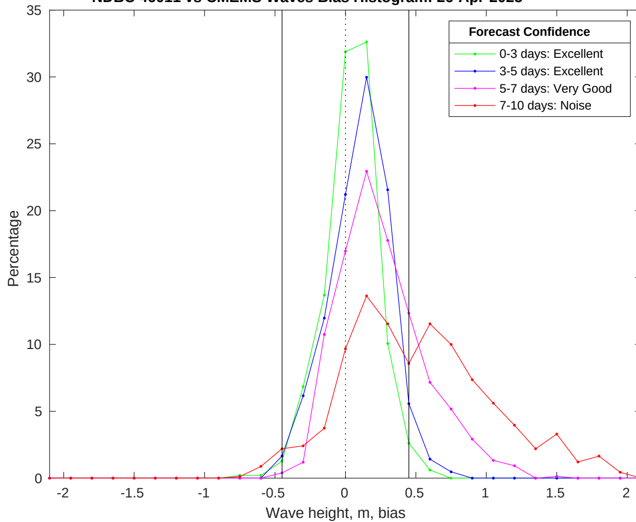
NDBC 46011 vs CMEMS Waves Bias Histogram: 26-Apr-2025
