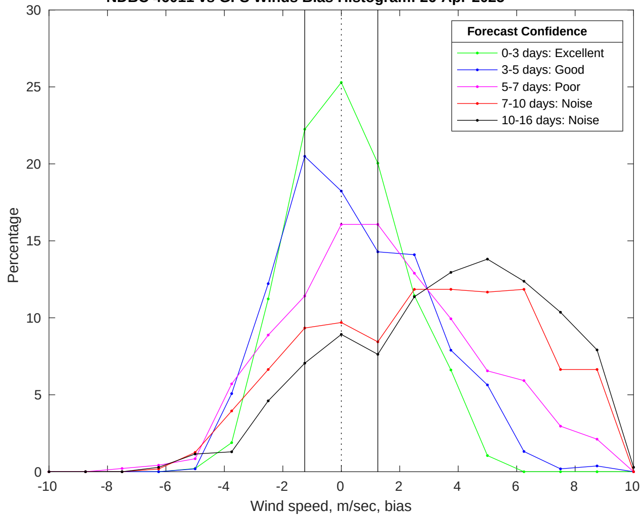
NDBC 46011 vs GFS Winds Bias Histogram: 26-Apr-2025
