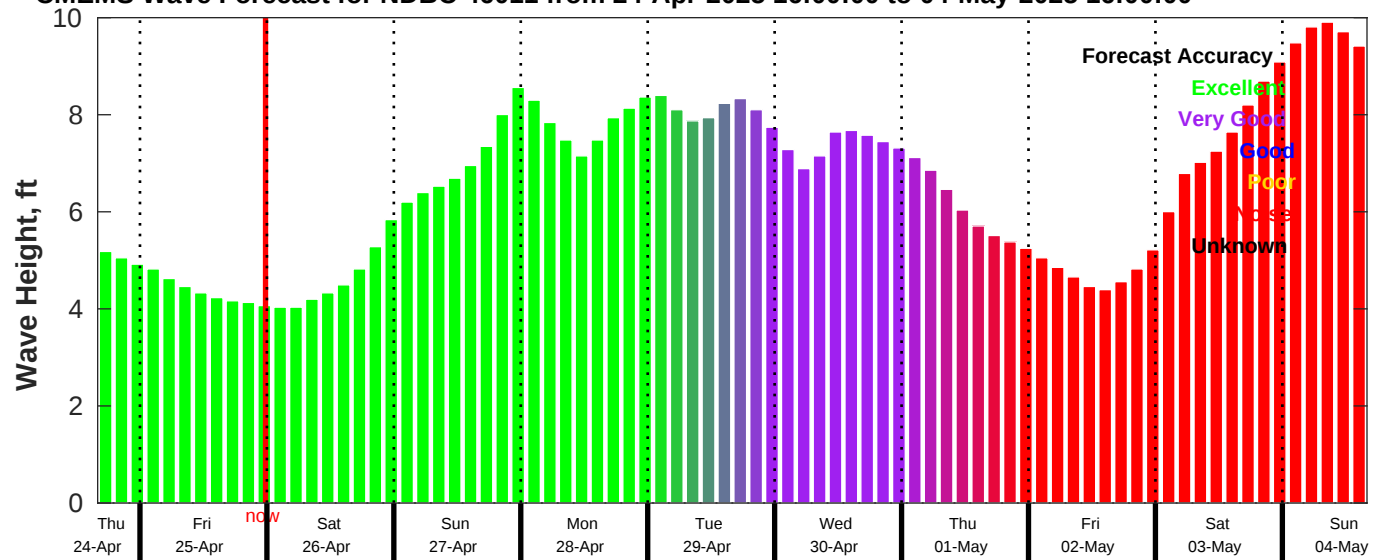
CMEMS Wave Forecast for NDBC 46011 from 24-Apr-2025 16:00:00 to 04-May-2025 16:00:00
