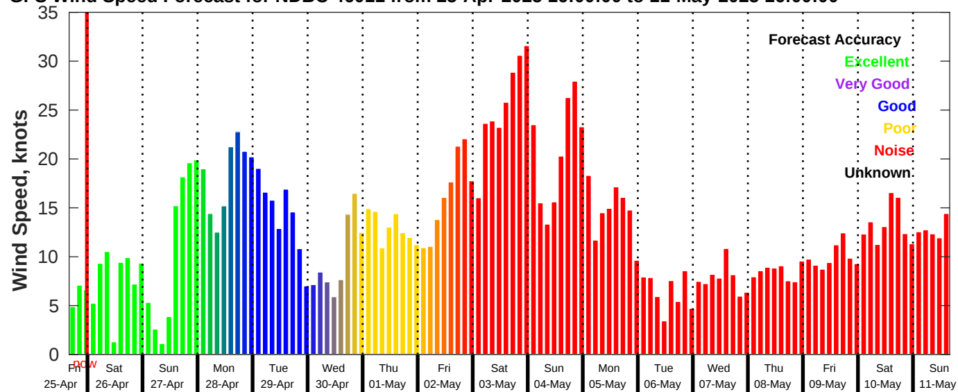
GFS Wind Speed Forecast for NDBC 46011 from 25-Apr-2025 16:00:00 to 11-May-2025 16:00:00
