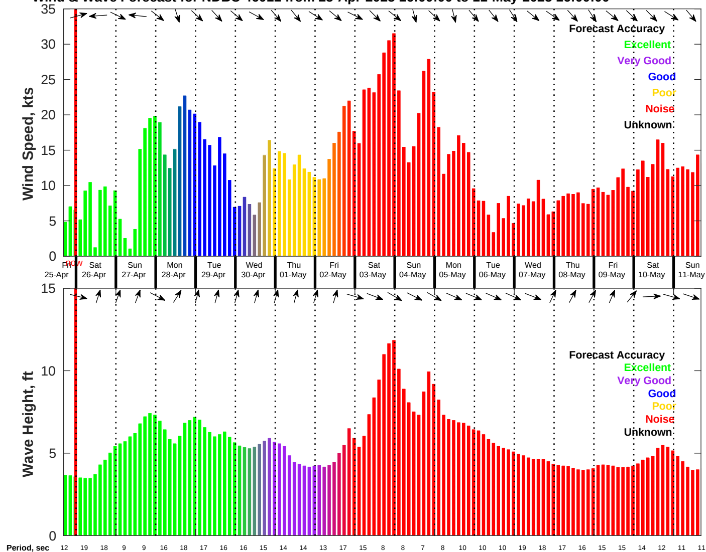
Wind & Wave Forecast for NDBC 46011 from 25-Apr-2025 16:00:00 to 11-May-2025 16:00:00
