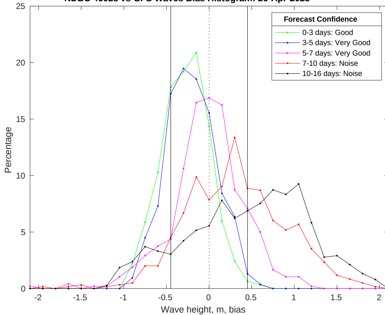
NDBC 46028 vs GFS Waves Bias Histogram: 26-Apr-2025
