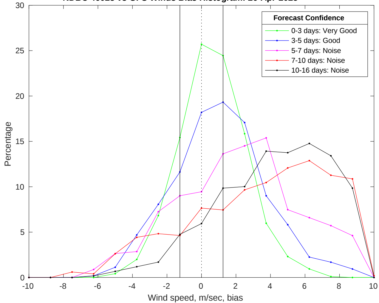
NDBC 46028 vs GFS Winds Bias Histogram: 26-Apr-2025
