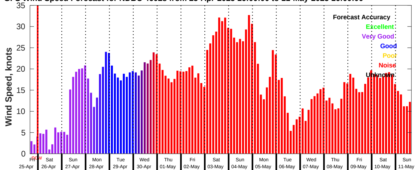
GFS Wind Speed Forecast for NDBC 46028 from 25-Apr-2025 16:00:00 to 11-May-2025 16:00:00
