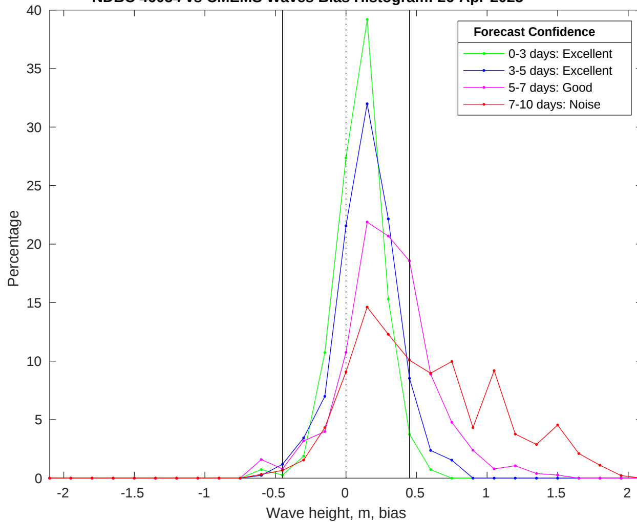
NDBC 46054 vs CMEMS Waves Bias Histogram: 26-Apr-2025
