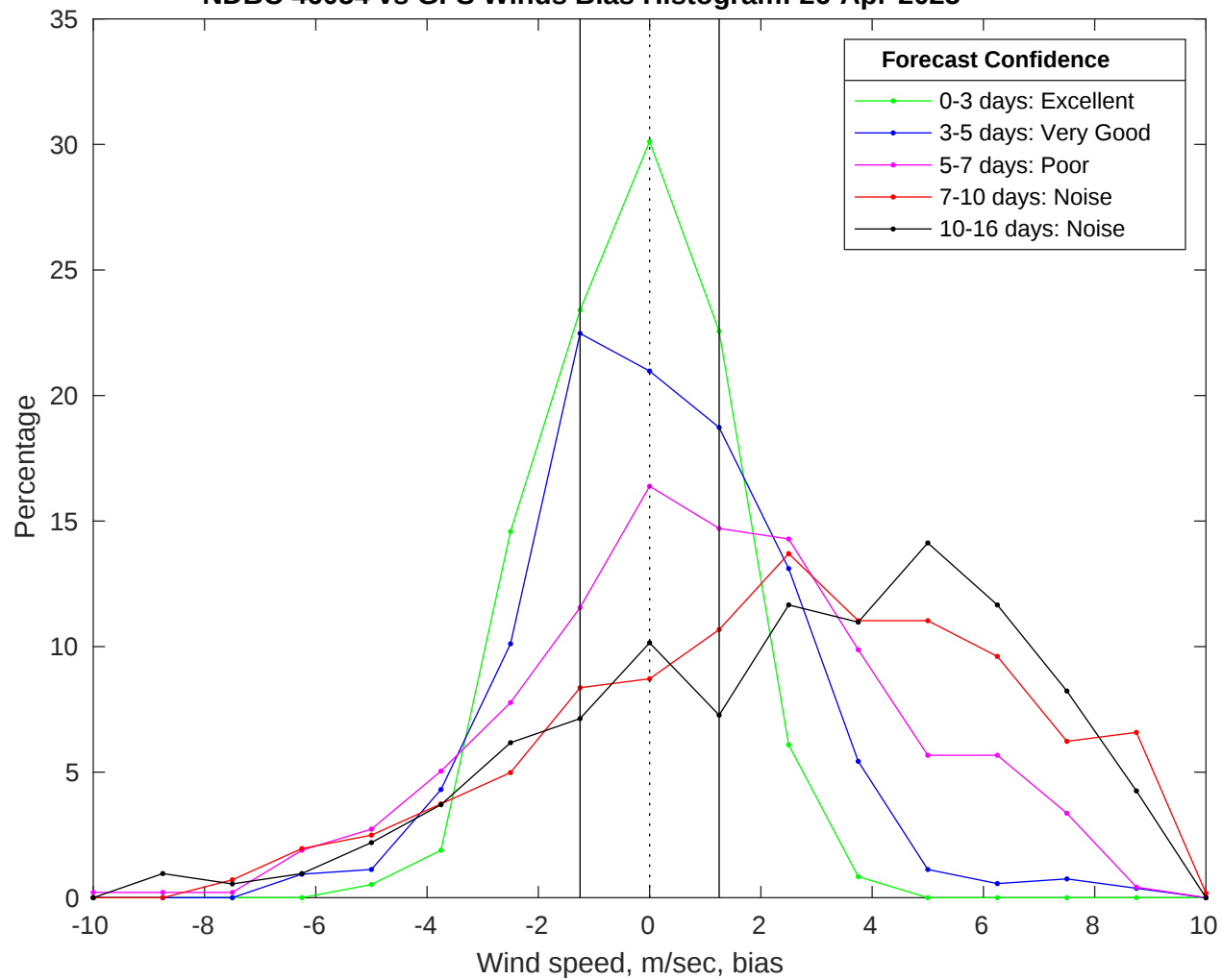
NDBC 46054 vs GFS Winds Bias Histogram: 26-Apr-2025
