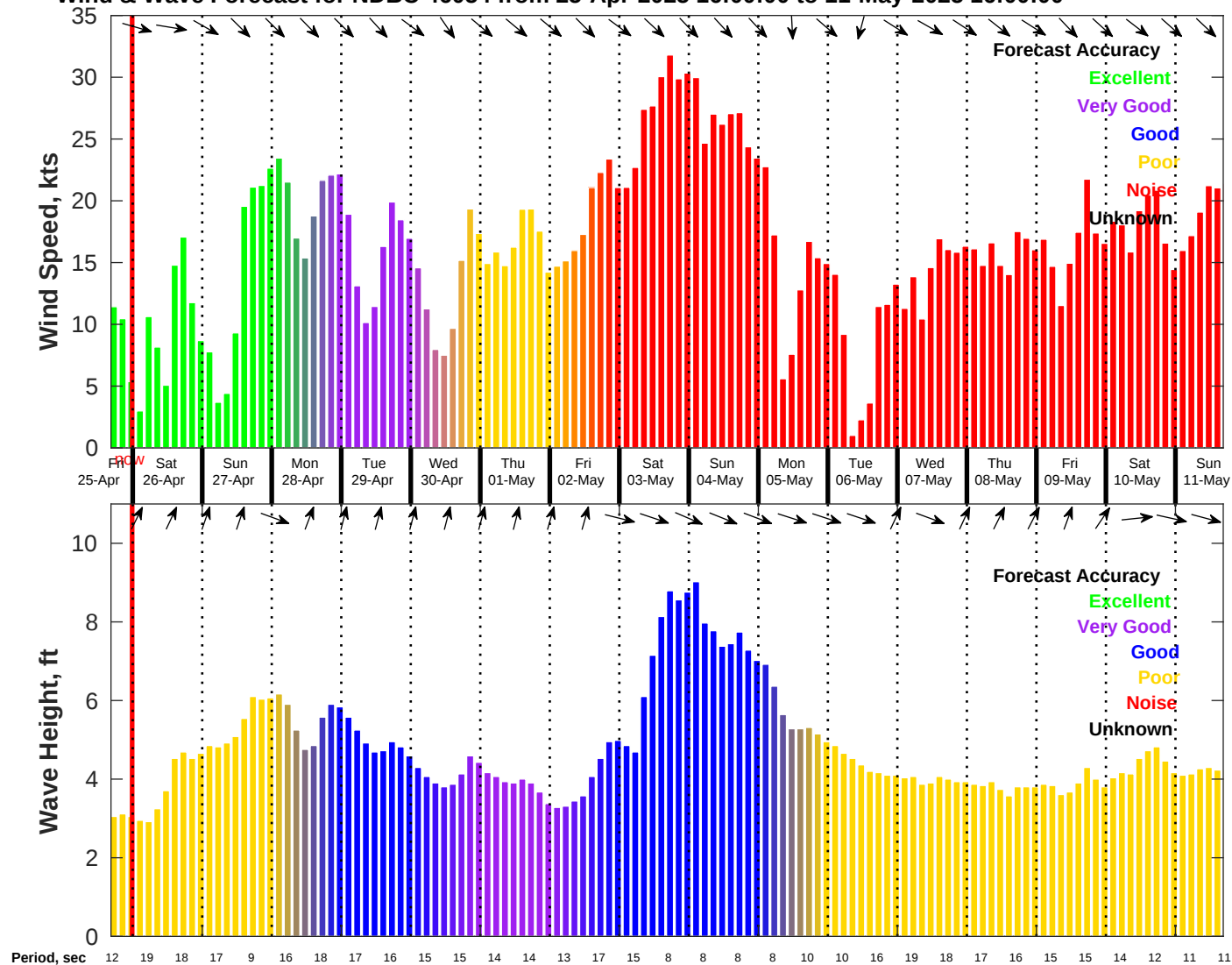
Wind & Wave Forecast for NDBC 46054 from 25-Apr-2025 16:00:00 to 11-May-2025 16:00:00
