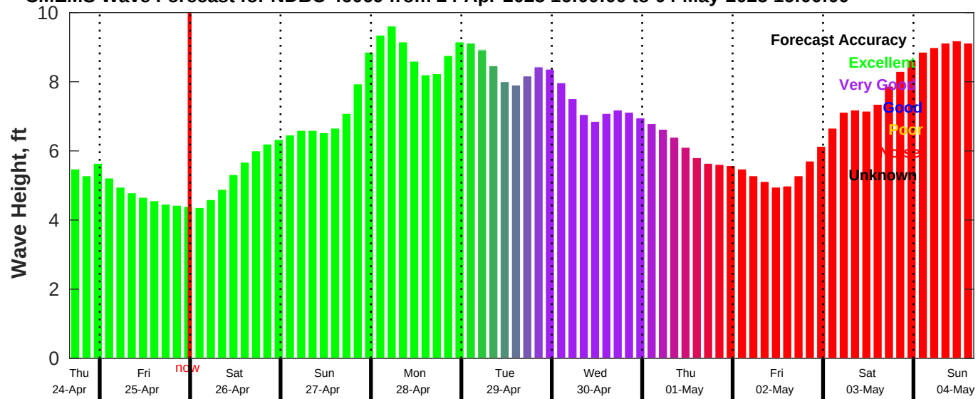
CMEMS Wave Forecast for NDBC 46069 from 24-Apr-2025 16:00:00 to 04-May-2025 16:00:00
