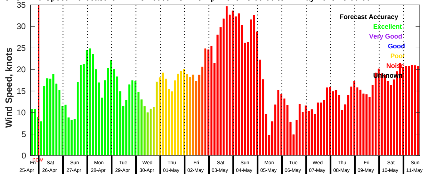
GFS Wind Speed Forecast for NDBC 46069 from 25-Apr-2025 16:00:00 to 11-May-2025 16:00:00
