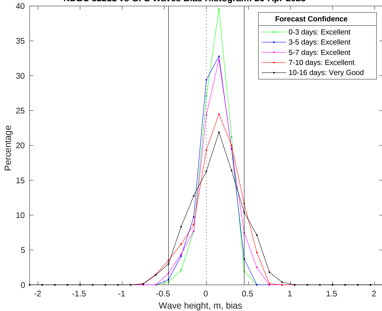
NDBC 52211 vs GFS Waves Bias Histogram: 26-Apr-2025
