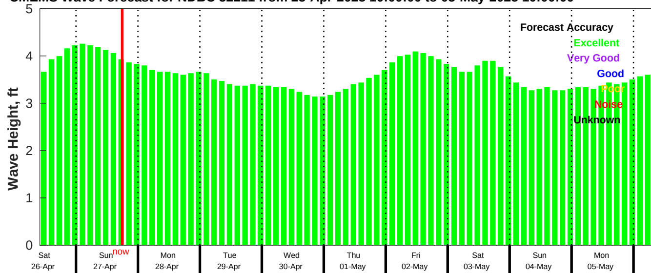
CMEMS Wave Forecast for NDBC 52211 from 25-Apr-2025 10:00:00 to 05-May-2025 10:00:00
