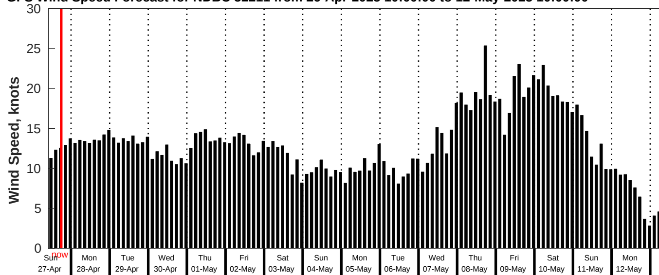
GFS Wind Speed Forecast for NDBC 52211 from 26-Apr-2025 10:00:00 to 12-May-2025 10:00:00
