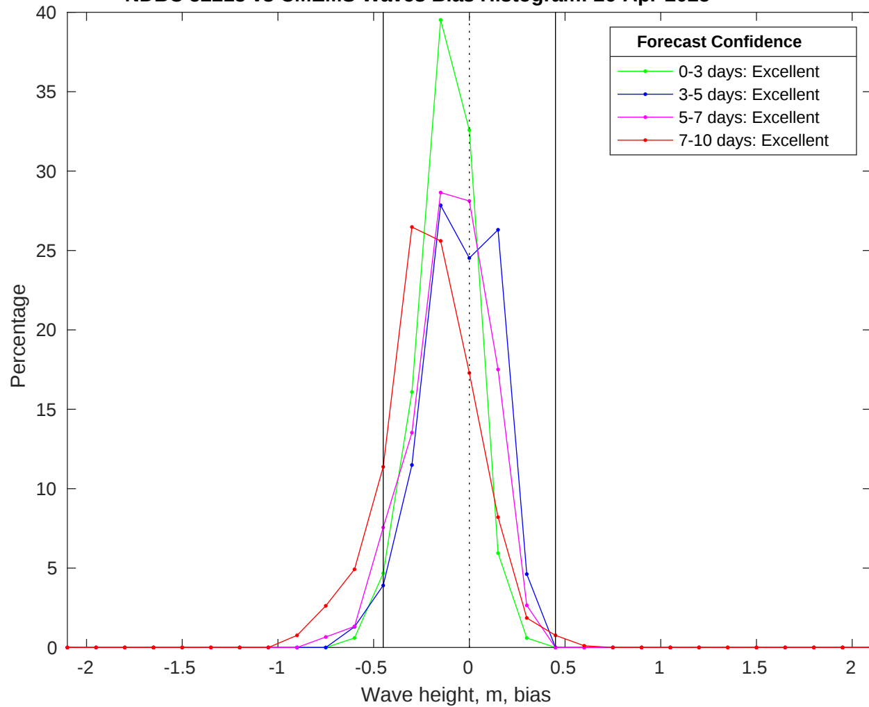
NDBC 52213 vs CMEMS Waves Bias Histogram: 26-Apr-2025
