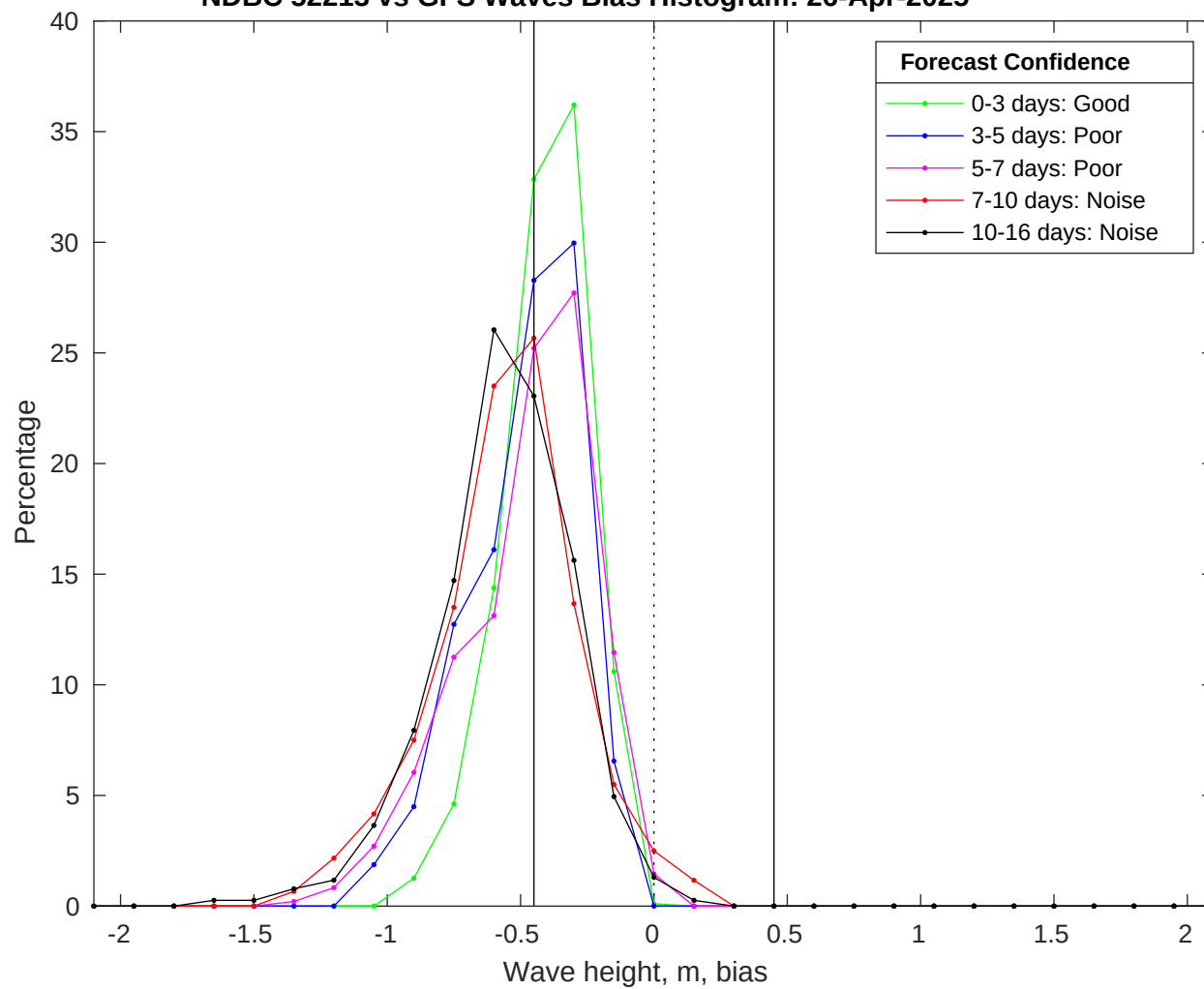
NDBC 52213 vs GFS Waves Bias Histogram: 26-Apr-2025
