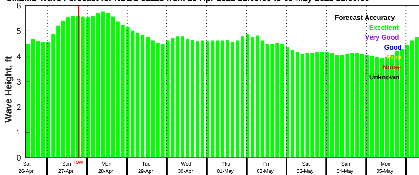
CMEMS Wave Forecast for NDBC 52213 from 25-Apr-2025 11:00:00 to 05-May-2025 11:00:00
