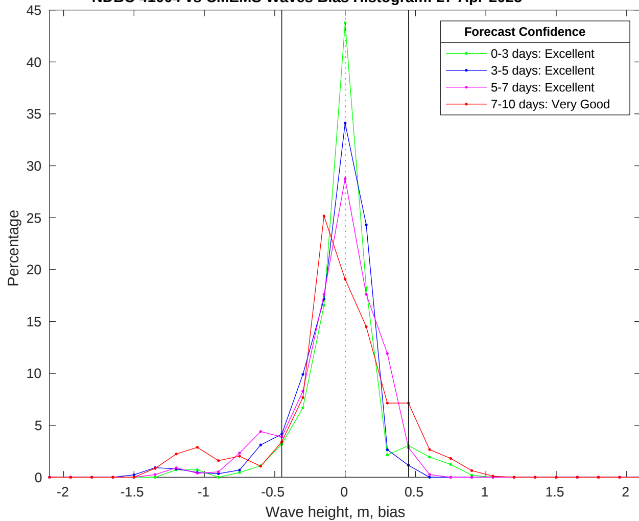
NDBC 41004 vs CMEMS Waves Bias Histogram: 27-Apr-2025
