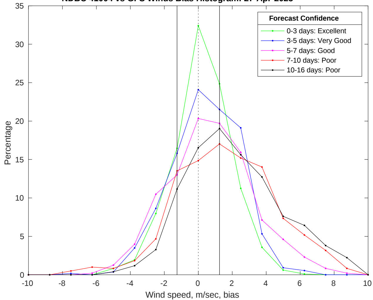
NDBC 41004 vs GFS Winds Bias Histogram: 27-Apr-2025
