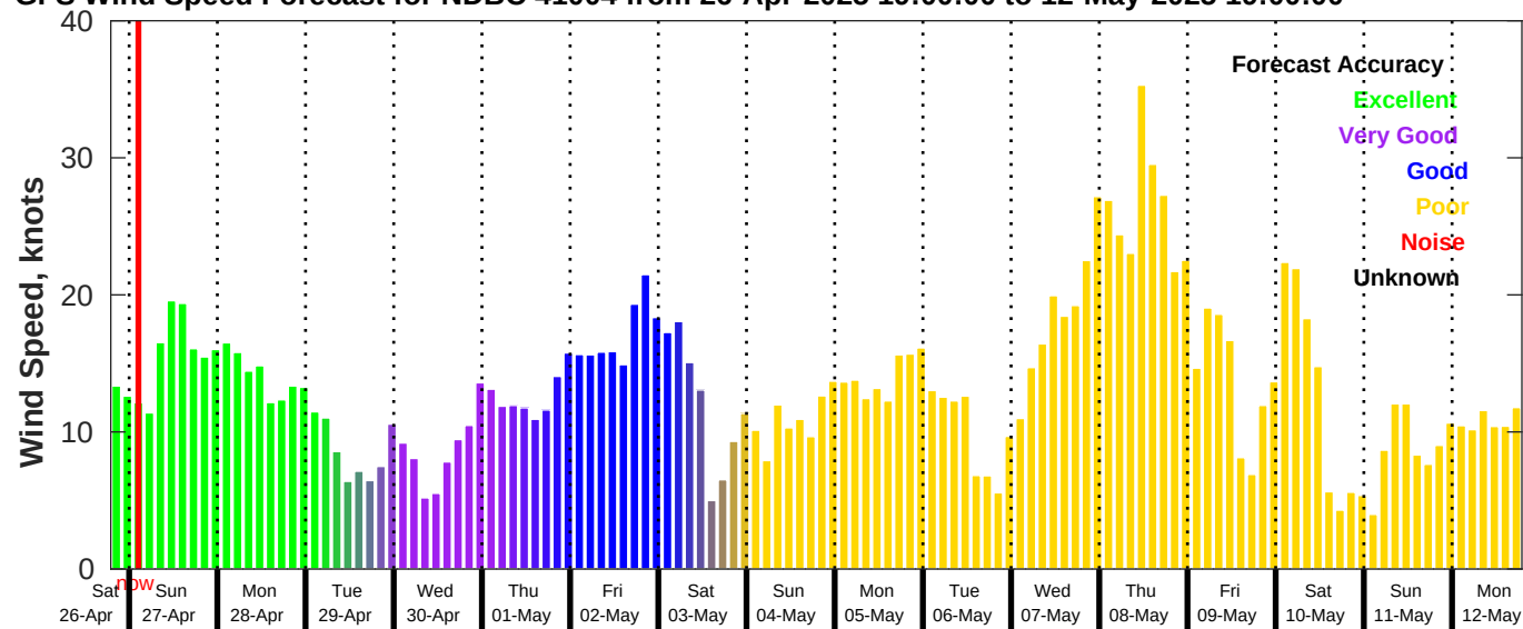
GFS Wind Speed Forecast for NDBC 41004 from 26-Apr-2025 19:00:00 to 12-May-2025 19:00:00
