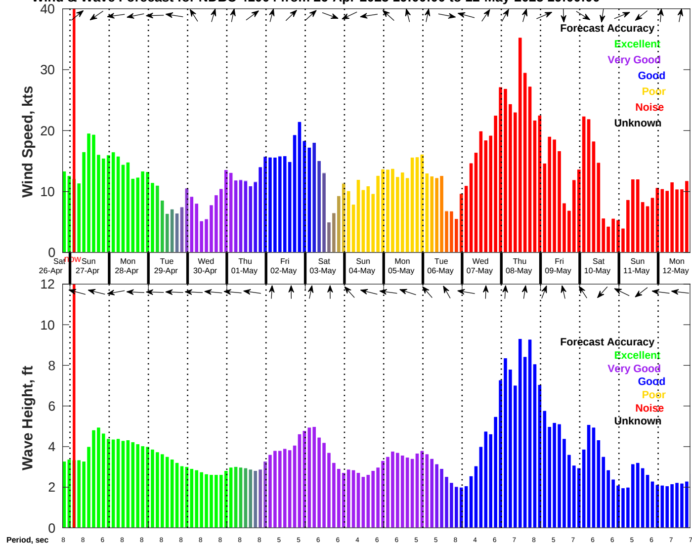
Wind & Wave Forecast for NDBC 41004 from 26-Apr-2025 19:00:00 to 12-May-2025 19:00:00
