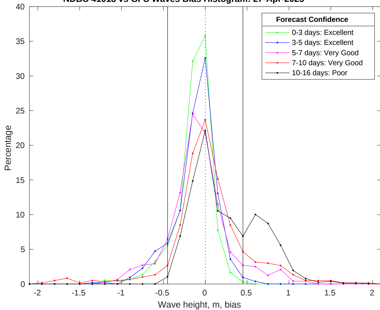
NDBC 41013 vs GFS Waves Bias Histogram: 27-Apr-2025
