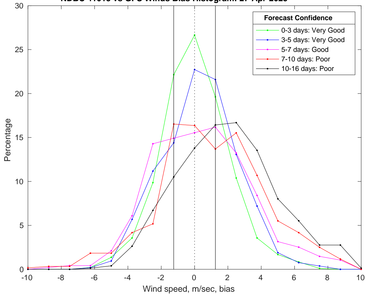
NDBC 41013 vs GFS Winds Bias Histogram: 27-Apr-2025
