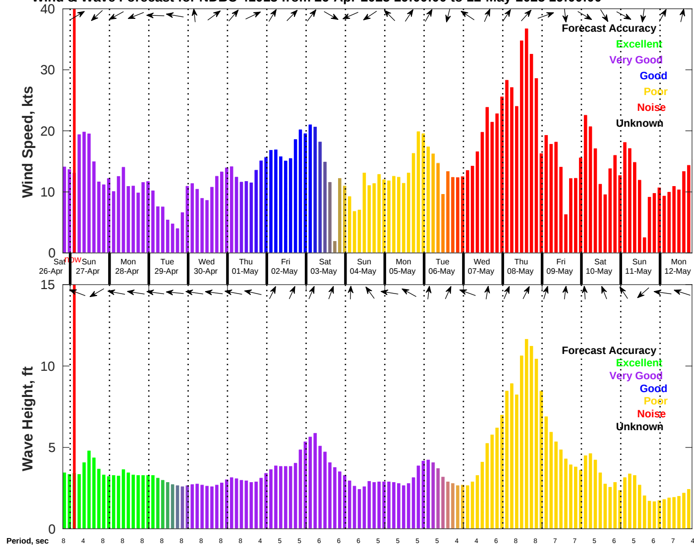
Wind & Wave Forecast for NDBC 41013 from 26-Apr-2025 19:00:00 to 12-May-2025 19:00:00
