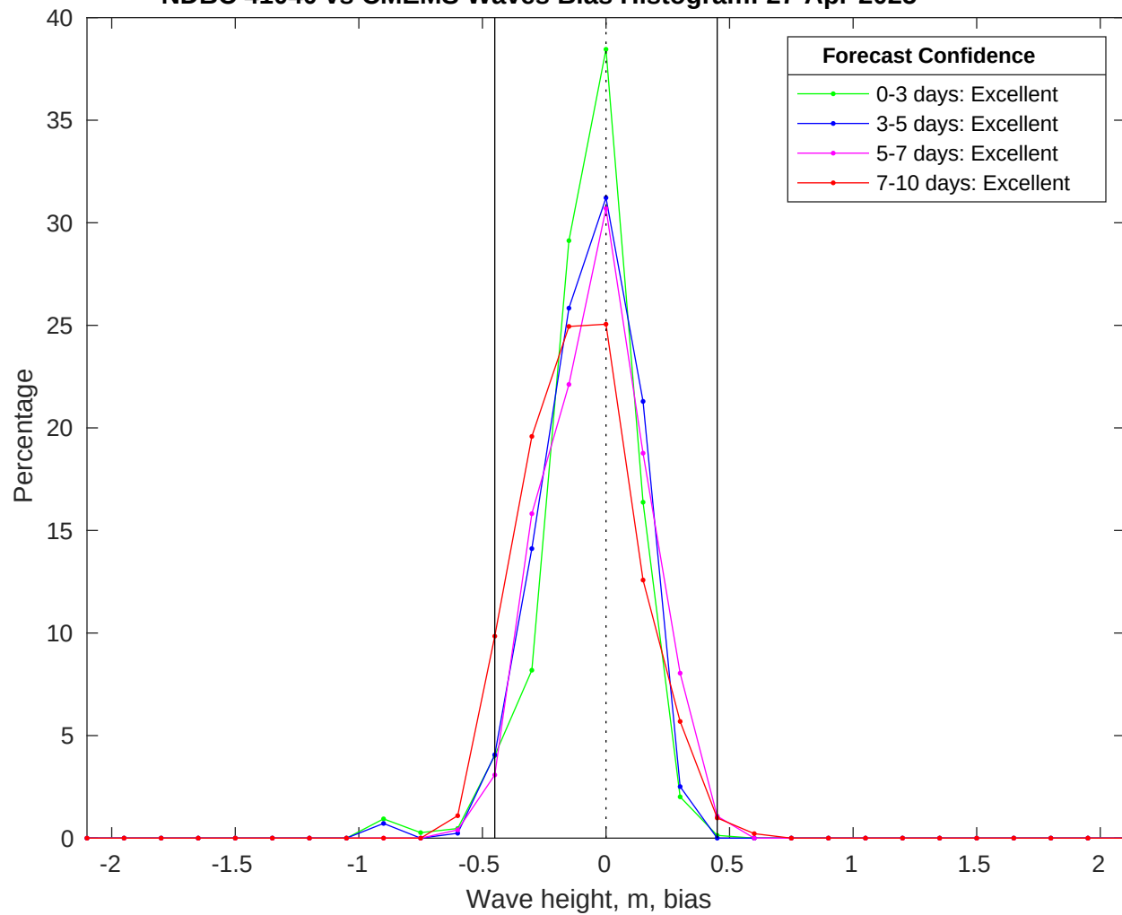
NDBC 41040 vs CMEMS Waves Bias Histogram: 27-Apr-2025
