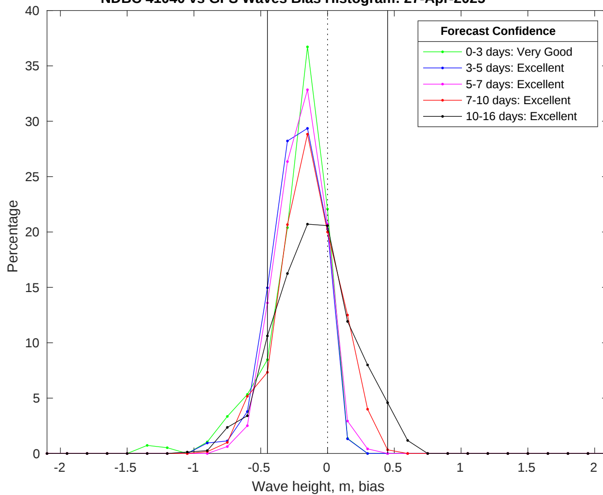
NDBC 41040 vs GFS Waves Bias Histogram: 27-Apr-2025
