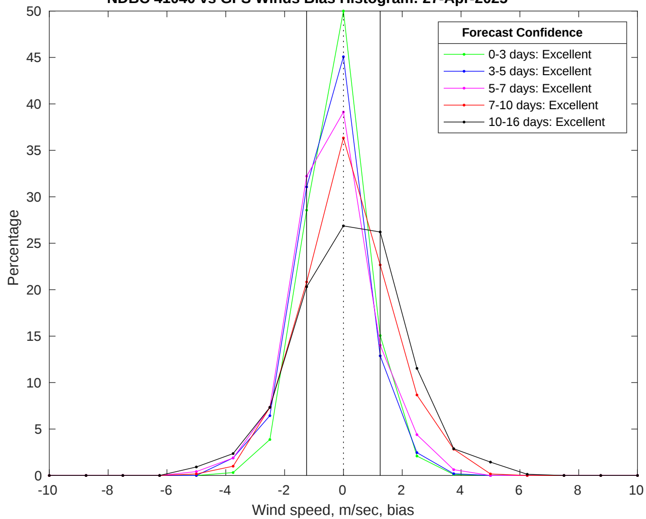
NDBC 41040 vs GFS Winds Bias Histogram: 27-Apr-2025
