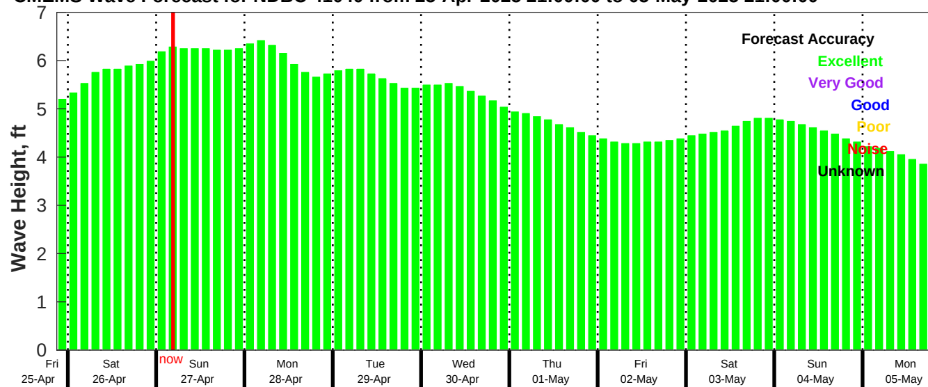
CMEMS Wave Forecast for NDBC 41040 from 25-Apr-2025 21:00:00 to 05-May-2025 21:00:00
