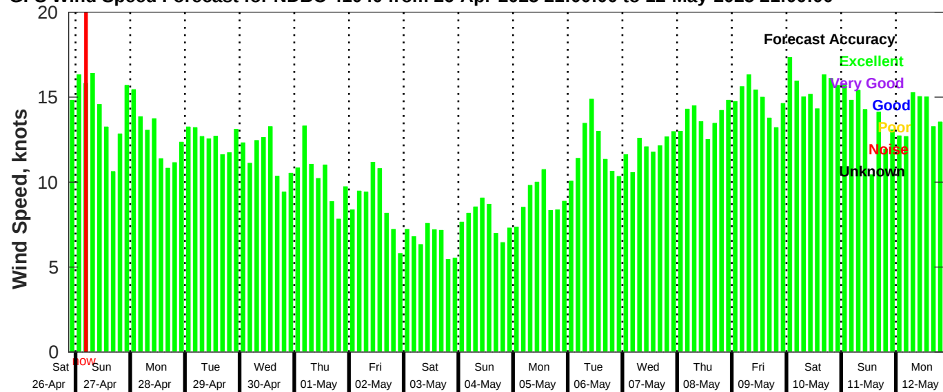
GFS Wind Speed Forecast for NDBC 41040 from 26-Apr-2025 21:00:00 to 12-May-2025 21:00:00
