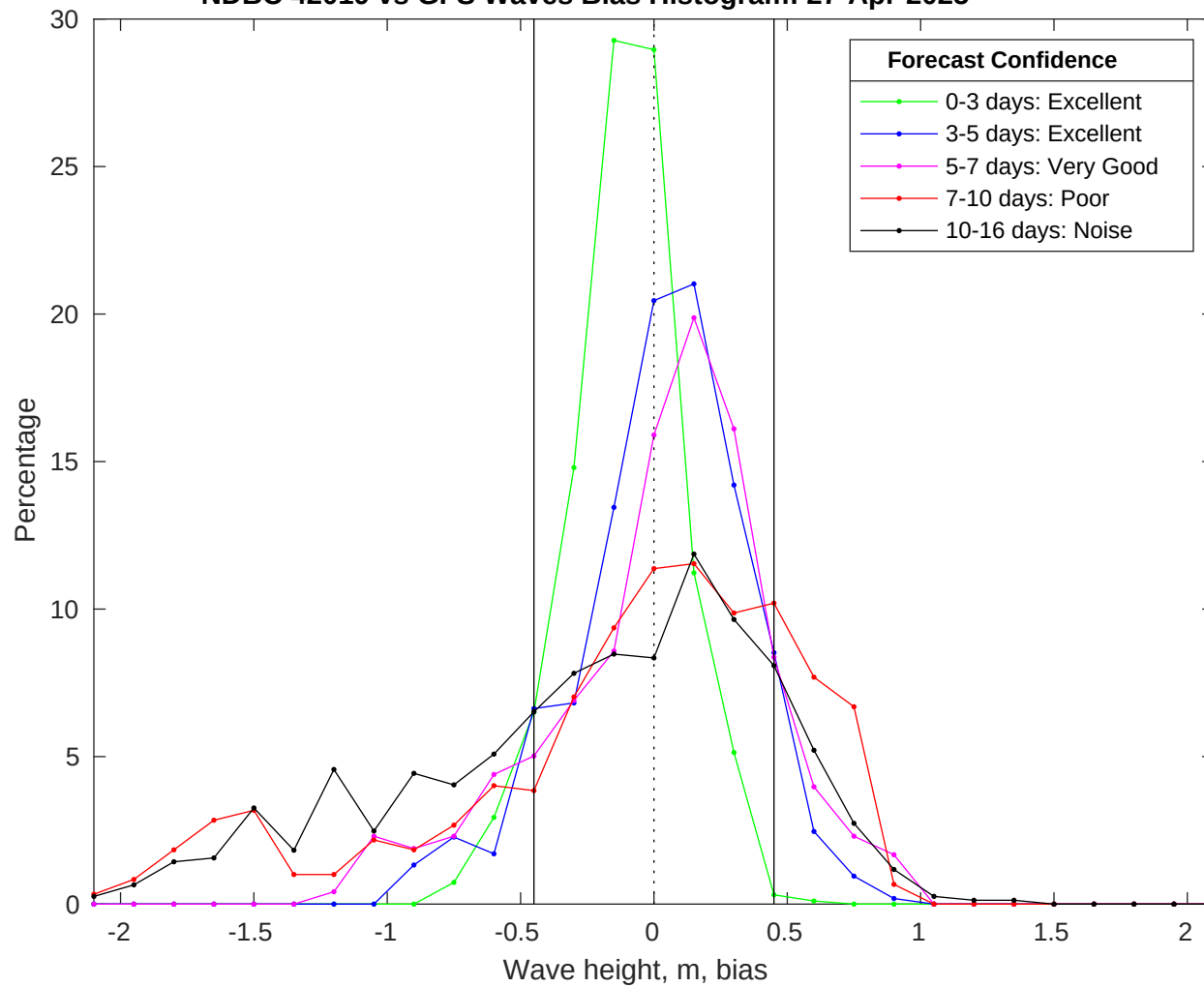
NDBC 42019 vs GFS Waves Bias Histogram: 27-Apr-2025
