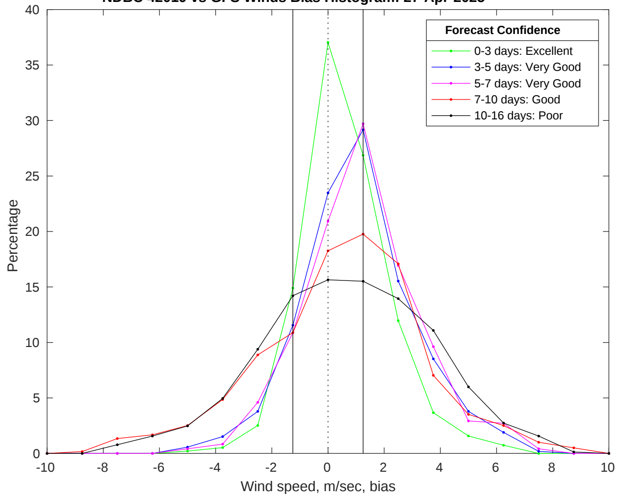
NDBC 42019 vs GFS Winds Bias Histogram: 27-Apr-2025
