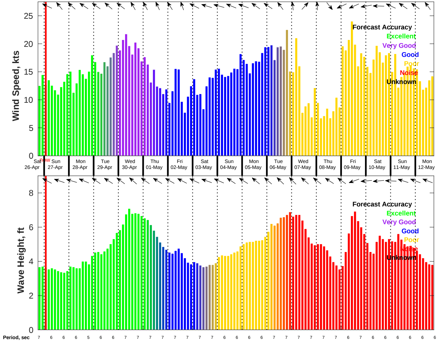
Wind & Wave Forecast for NDBC 42019 from 26-Apr-2025 18:00:00 to 12-May-2025 18:00:00
